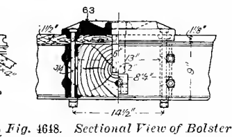
Fig. 4648. Sectional View of Bolster.
